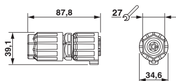
Dimensional drawing: connector, 2.5 mm²
