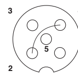
Pin assignment socket M 12, 3-pos. + PE
