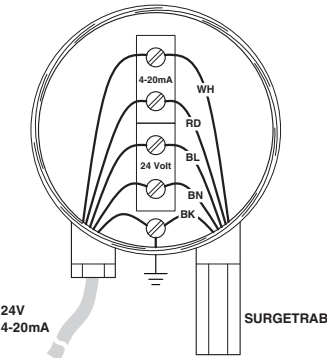
Application drawing
