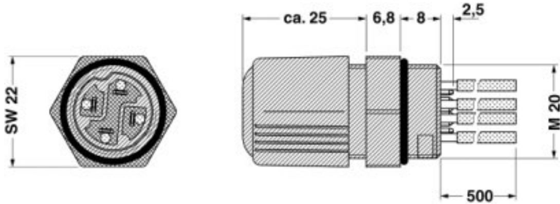
Dimensioned drawing
