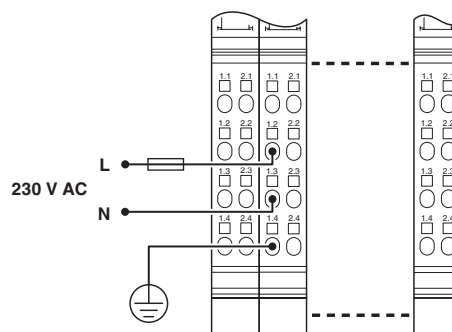
Figure 4 Typical connection of the supply voltage
