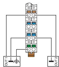
Connection diagram
