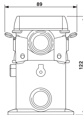
Dimensional drawing
