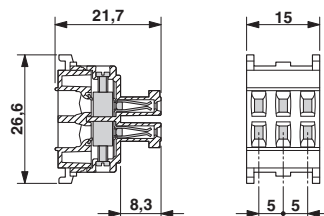
Dimensioned drawing
