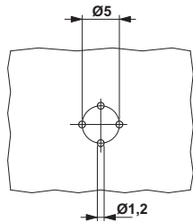
M12 flush-type connector
