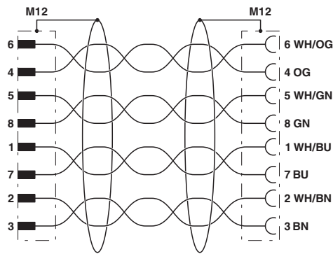
Contact assignment of the M12 connector and the M12 socket
