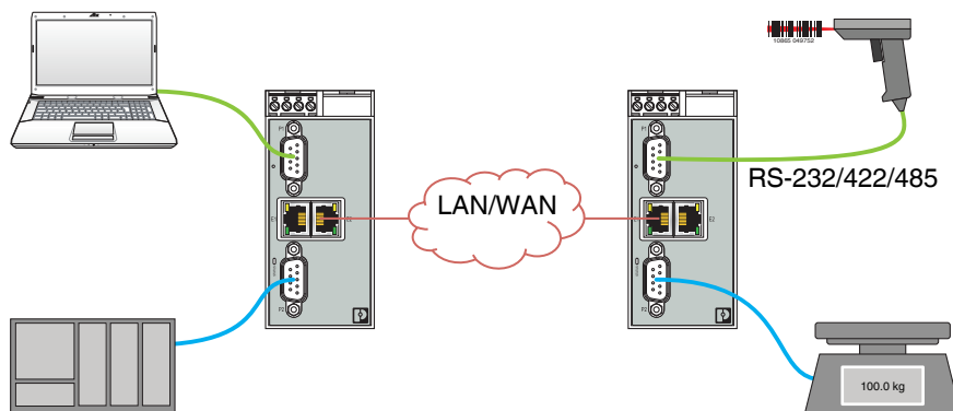
Figure 4 Serial tunneling
