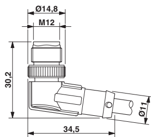
M12 x 1 male connector, angled
