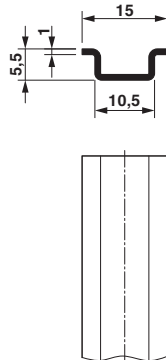
Dimensional drawing
