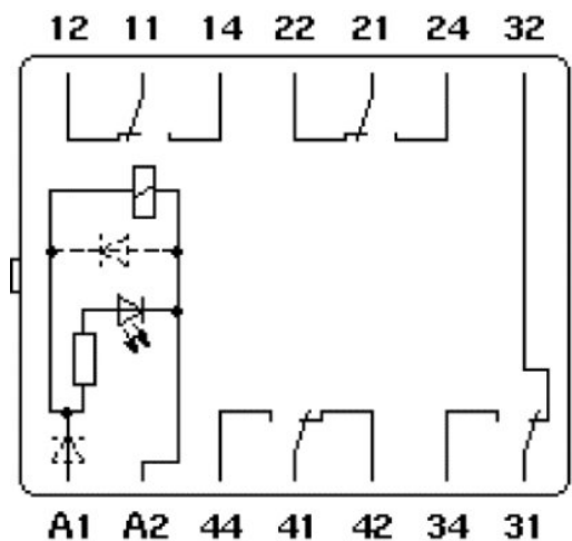
Circuit diagram
