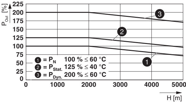
Figure 30 Output power depending on the installation height
