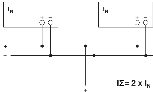
Figure 28 Schematic diagram of increased performance
