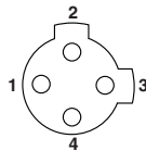
Pin assignment 1/2"-20UNF socket, 4-pos., view female side
