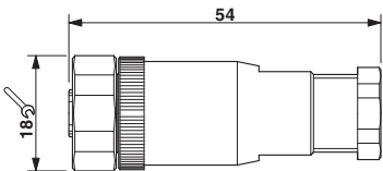
Dimensioned drawing
