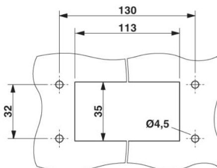
Panel cutout
