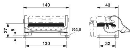
Dimensional drawing
