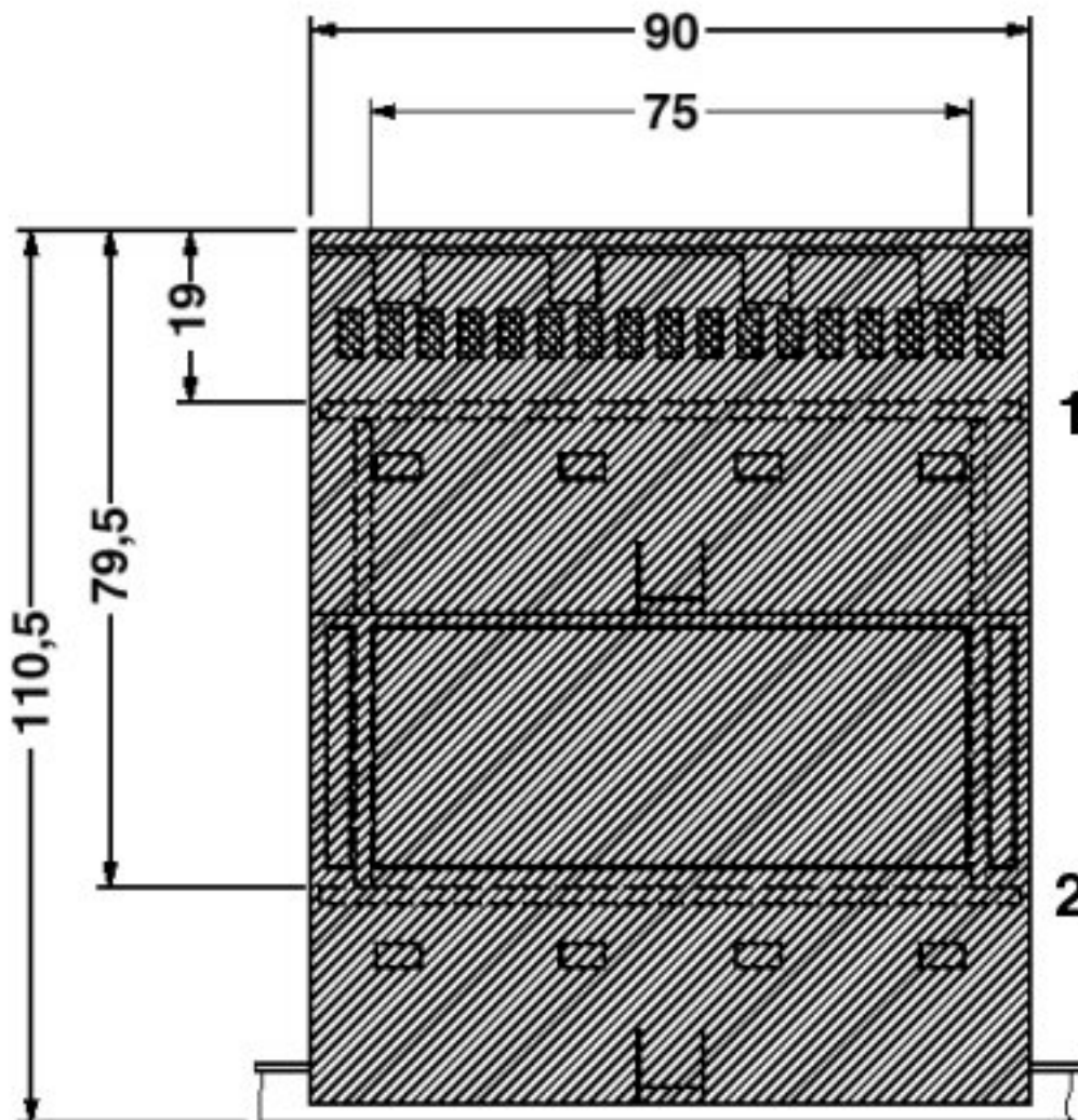
Dimensioned drawing
