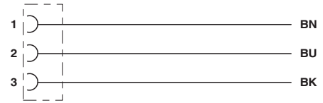
Contact assignment of the DEUTSCH DT06-3S
