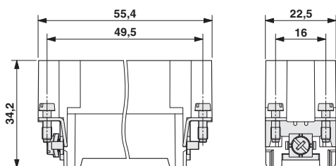
Male insert
