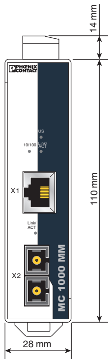
Figure 1 Housing dimensions
