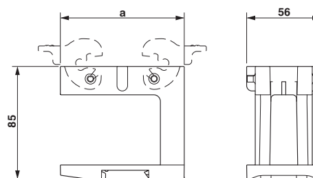
Dimensional drawing, a = 93.5 mm
