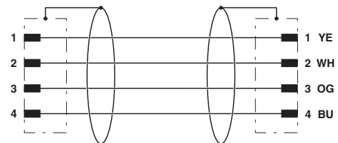
Contact assignment of M8 plugs
