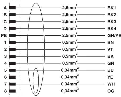
Contact assignment of M23 plugs/sockets
