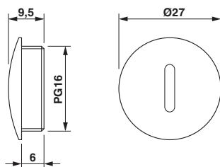
Dimensional drawing
