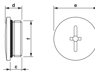
Dimensional drawing
