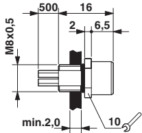
M8 flush-type socket
