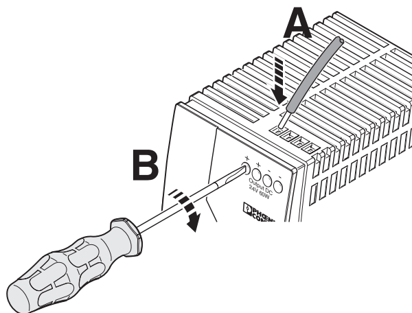
Figure 10 Connecting cables
