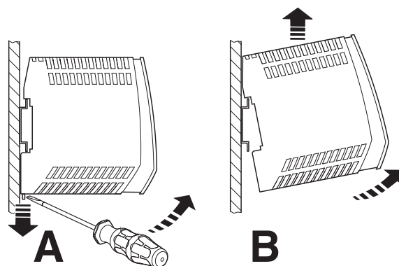
Figure 15 Removal
