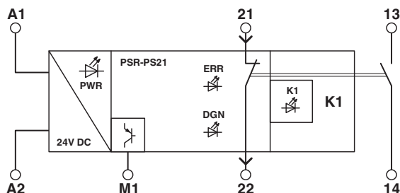
Figure 1 Block diagram
