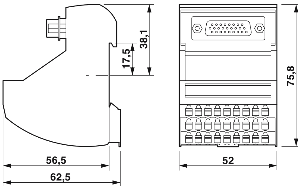
Dimensional drawing
