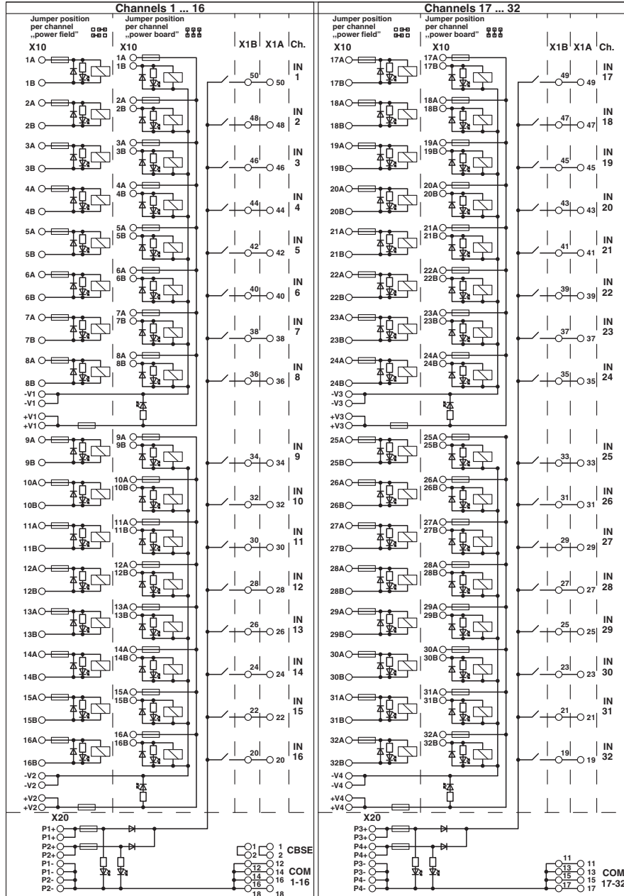
Circuit diagram
