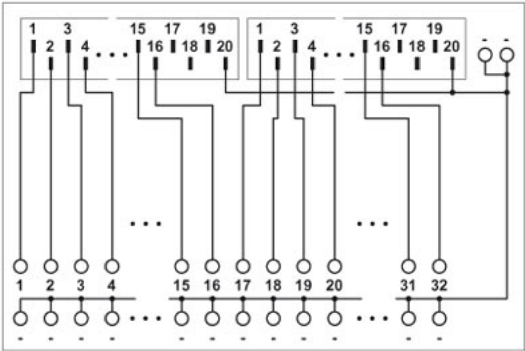
Connection diagram
