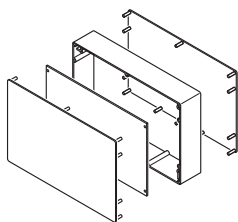
Exploded view
