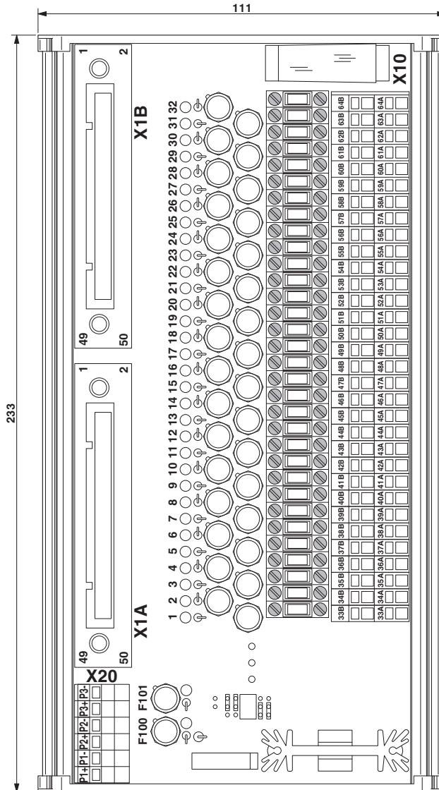
Dimensional drawing
