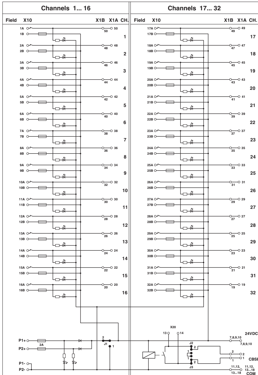
Circuit diagram
