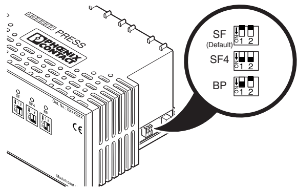
Figure 3 DIP switches
