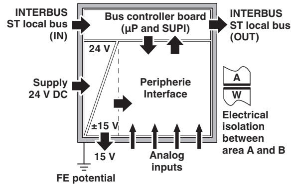
Figure 2 Electrical isolation of the individual function areas
