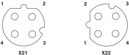
Figure 3 Pin assignment, D-coded
