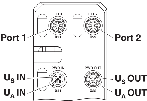
Figure 2 Connections for Sercos and power supply
