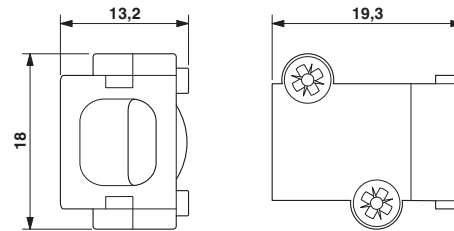
Dimensioned drawing
