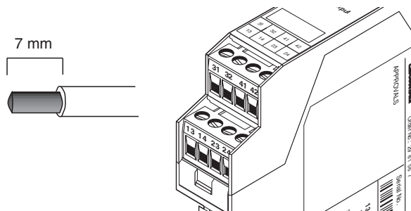
Figure 3 PSR-SCP- 24DC/SSM/2X1
