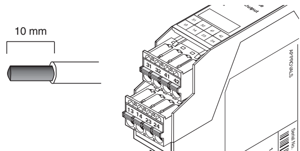
Figure 4 PSR-SPP- 24DC/SSM/2X1
