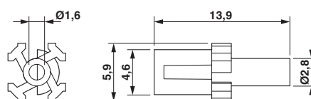
Schematic diagram
