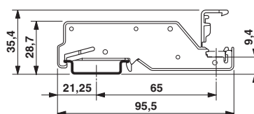
Dimensional drawing
