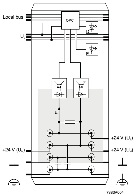
Figure 2 Internal wiring of the terminal points
