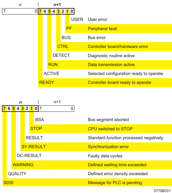
Figure 24 Diagnostic status register
