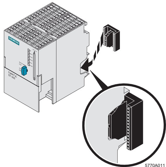
Figure 12 Inserting the bus connector
