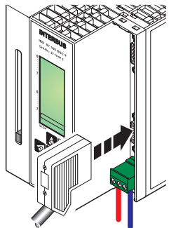
Figure 4 Remote bus connection
