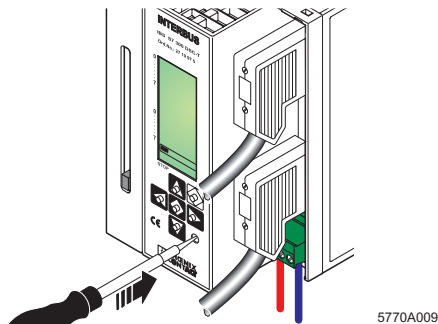
Figure 15 Test mode button
