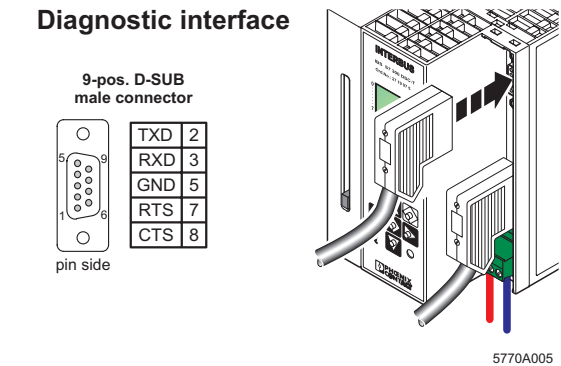
Figure 6 Diagnostic interface
