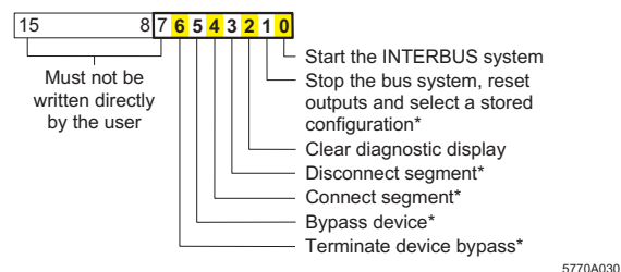
Figure 25 Assignment of frequently used functions in the standard function start register
