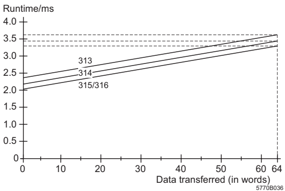
Figure 21 FC 22, Q area
