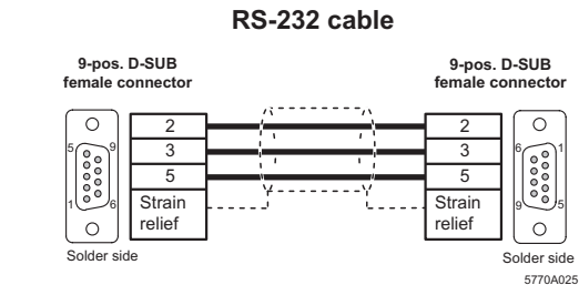
Figure 7 RS-232 cable for connection to a PC
