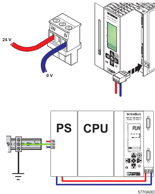
Figure 3 Connection of the external supply voltage
