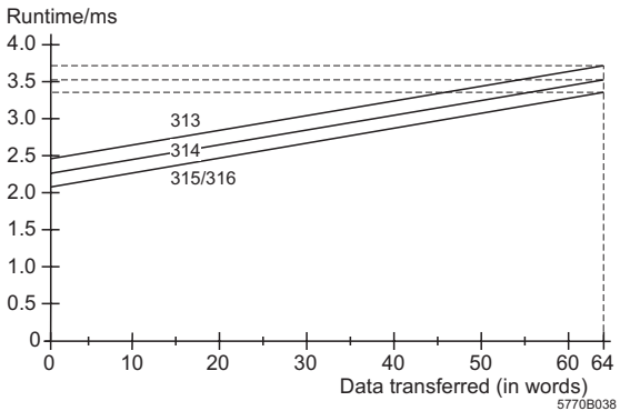
Figure 23 FC 22, data block area
