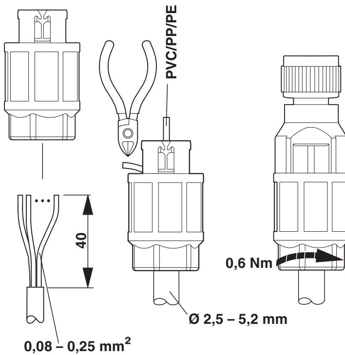
Functional drawing
