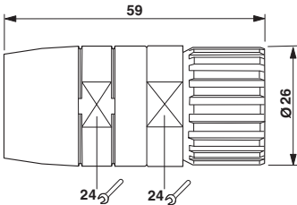
Dimensioned drawing
