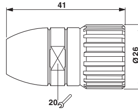
Dimensioned drawing
