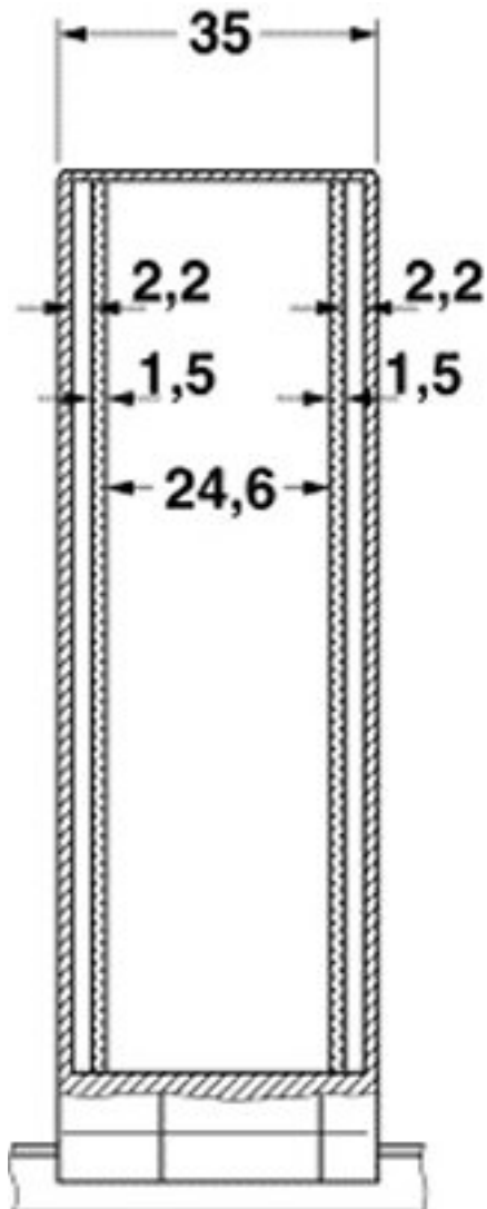
Dimensioned drawing
