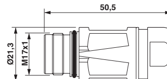
Dimensioned drawing
