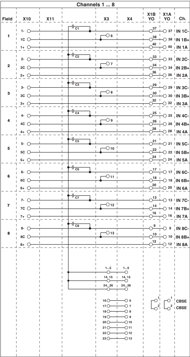
Circuit diagram
