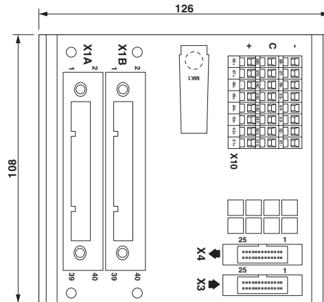
Dimensional drawing
