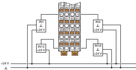
Connection diagram
