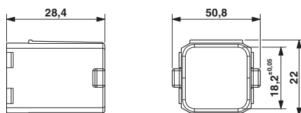
Protective cover
